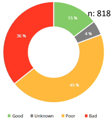
Figure 3.4 Conservation status of habitats at EU level
