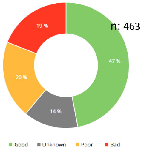
Figure 2.4 EU population status of bird species
